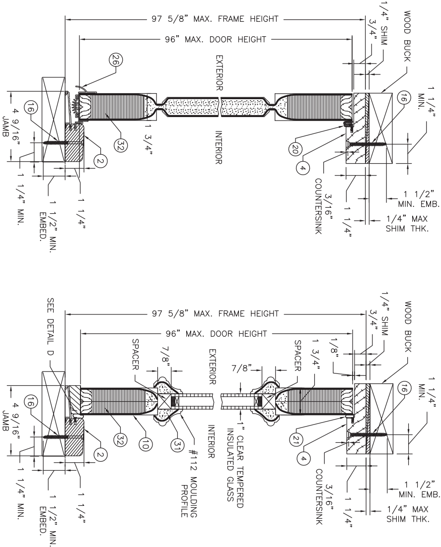
1 3 DOOR VERTICAL CROSS SECTION TYP. SCALE: 3" = 1'-0"
